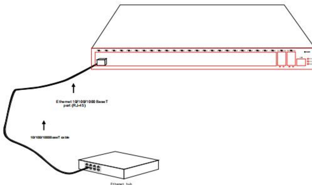
Figure 3-5 Gigabit SFP ports connect to other Ethernet terminal devices
