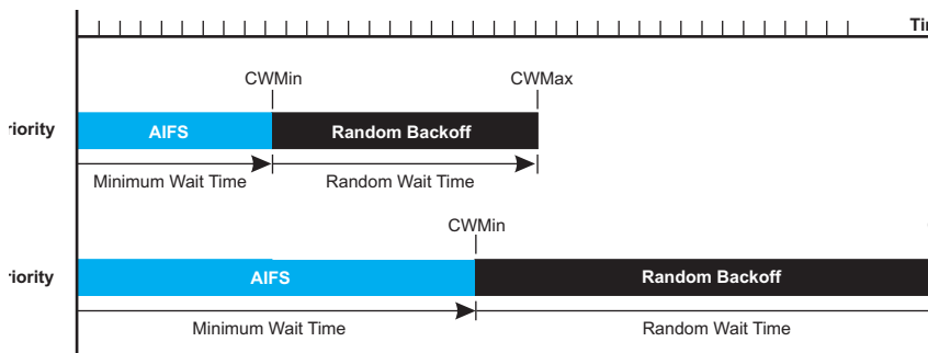
Figure 5-1. WMM Backoff Wait Times
