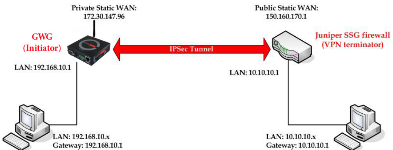
Figure 115 – IPSec tunnel between GWG Gateway and Juniper SSG
