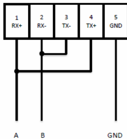
Figure 45- GWR RS-422/RS-485 Port Wiring
