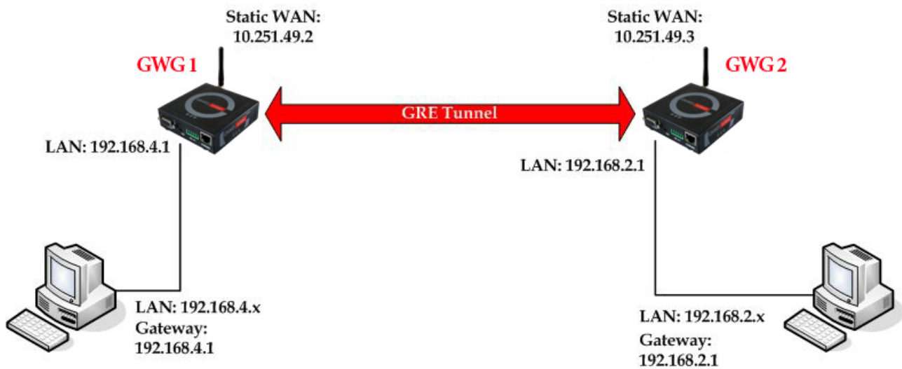
Figure 72 – GRE tunnel between two GWG Gateways
