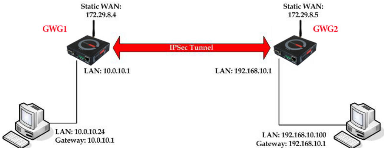
Figure 83 – IPSec tunnel between two GWG Gateways
