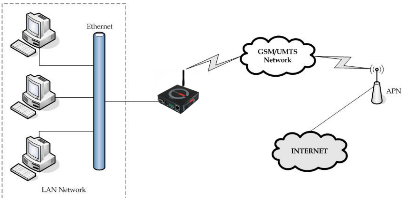
Figure 71 – GWG Gateway as Internet gateway
