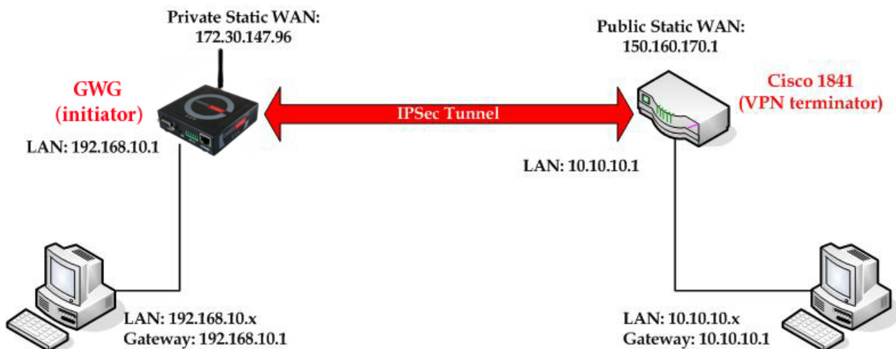
Figure 109 – IPSec tunnel between GWG Gateway and Cisco Router
