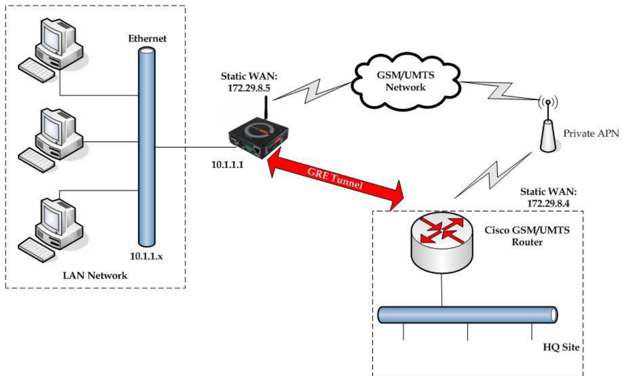
Figure 79 – GRE tunnel between Cisco router and GWG Gateway
